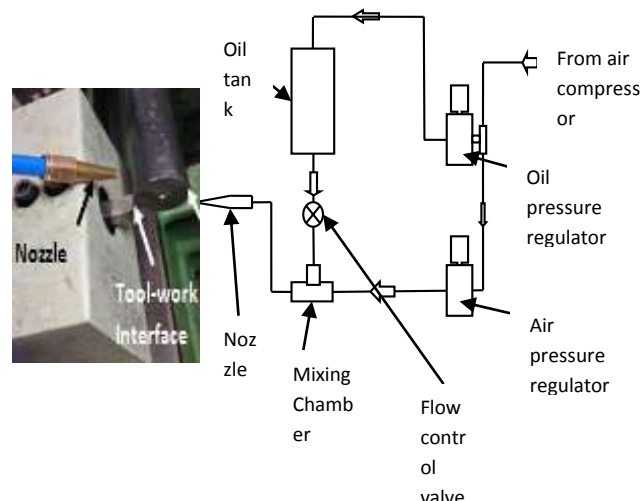
Fig. 1 MQL set-
